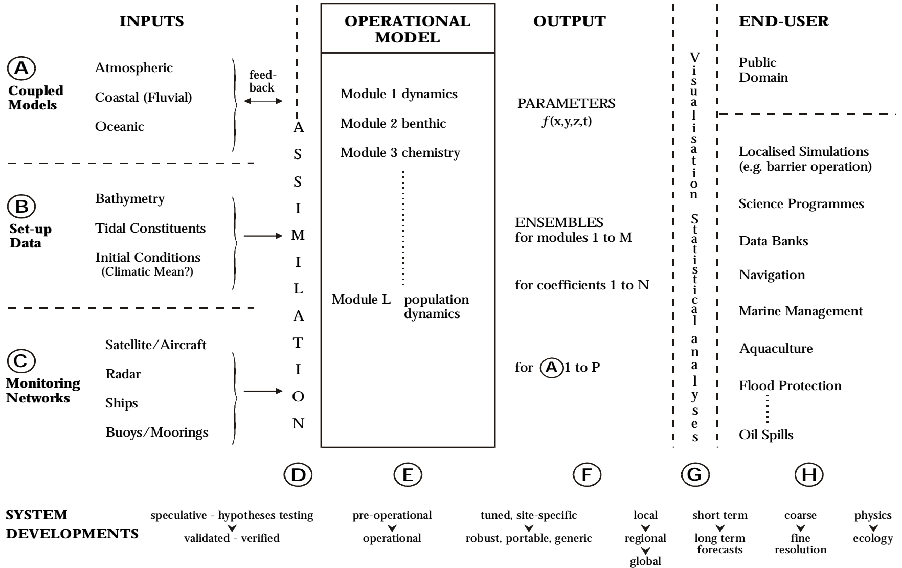
Figure 6. Components of Operational Oceanography (A) to (H) and future developments.
