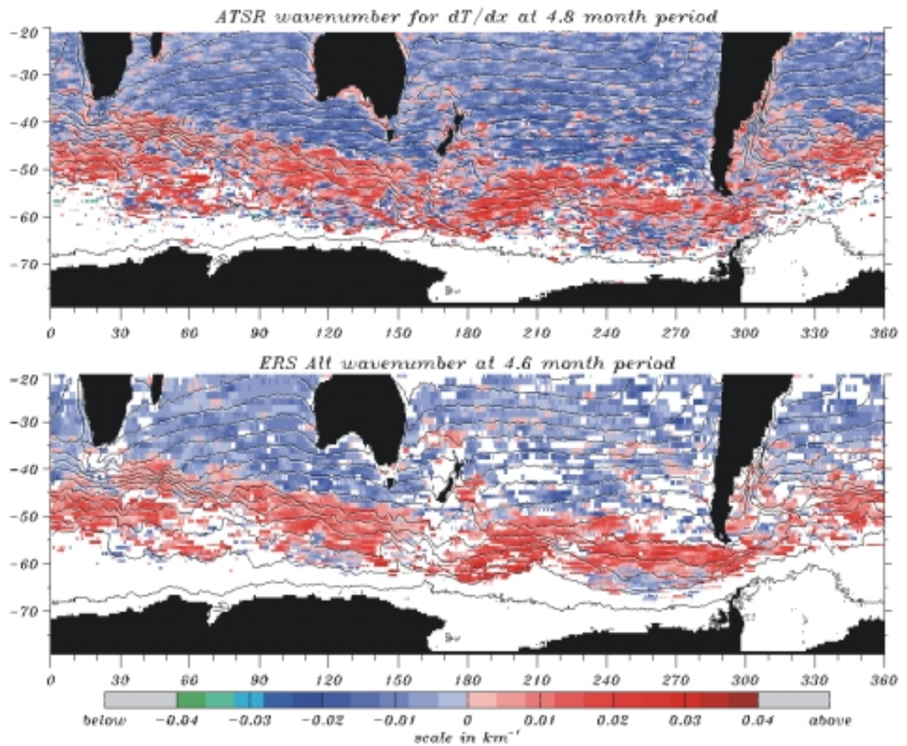
Figure 3. Global ATSR/ERS satellite data
