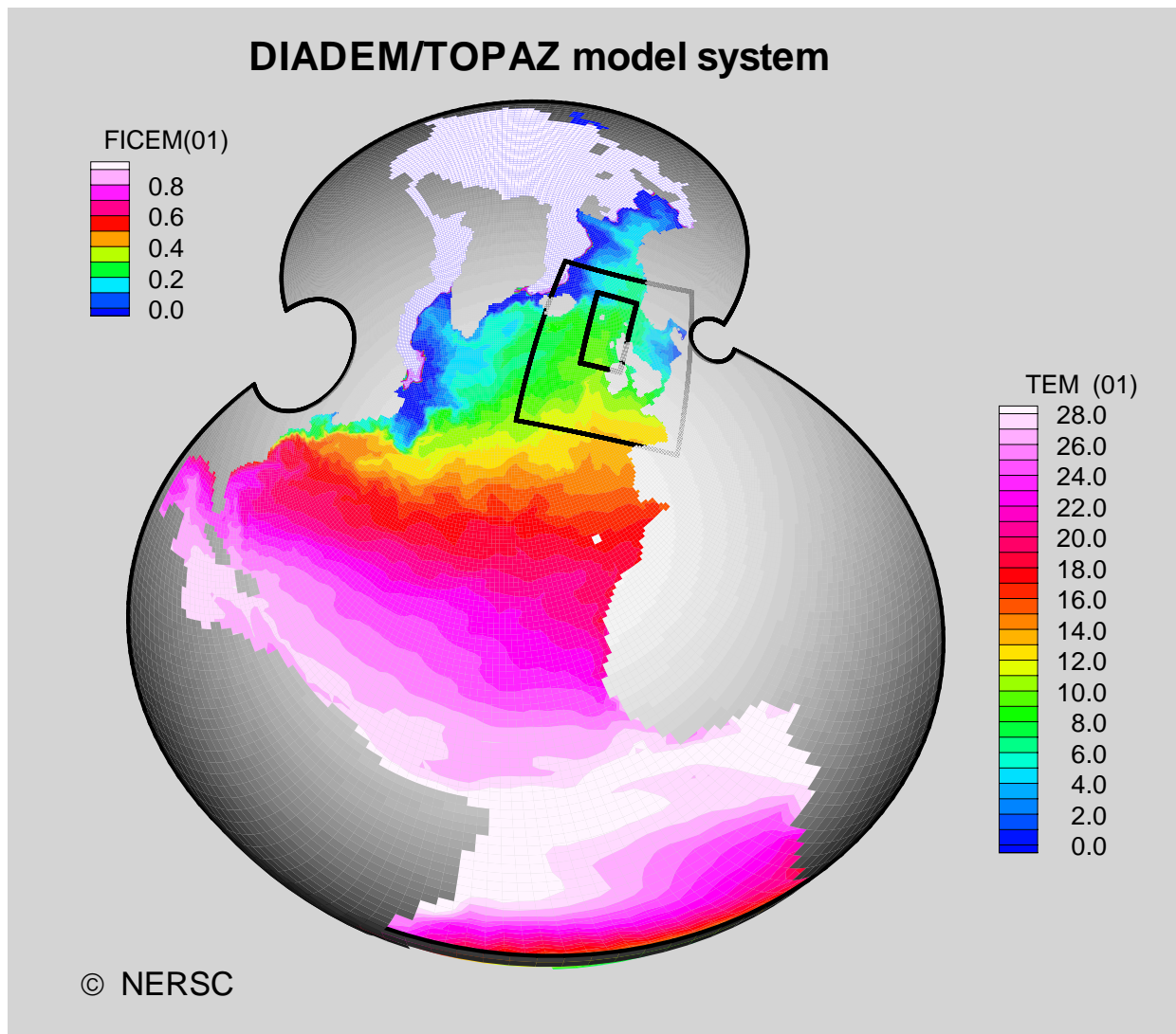
Figure 4: Modelling grid for the DIADEM/TOPAZ model showing a surface temperature field, and the high resolution zones where nested models will be run with resolution of 7-8km and 2km
