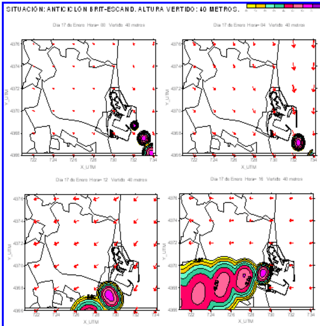
Figure 5: Particle Dispersion model. Unloading at east quay PA Valencia
