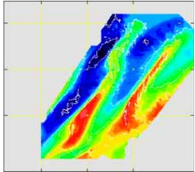
Figure 9: An example of bathymetric information derived from SAR imagery (supplied by ARGOSS)
