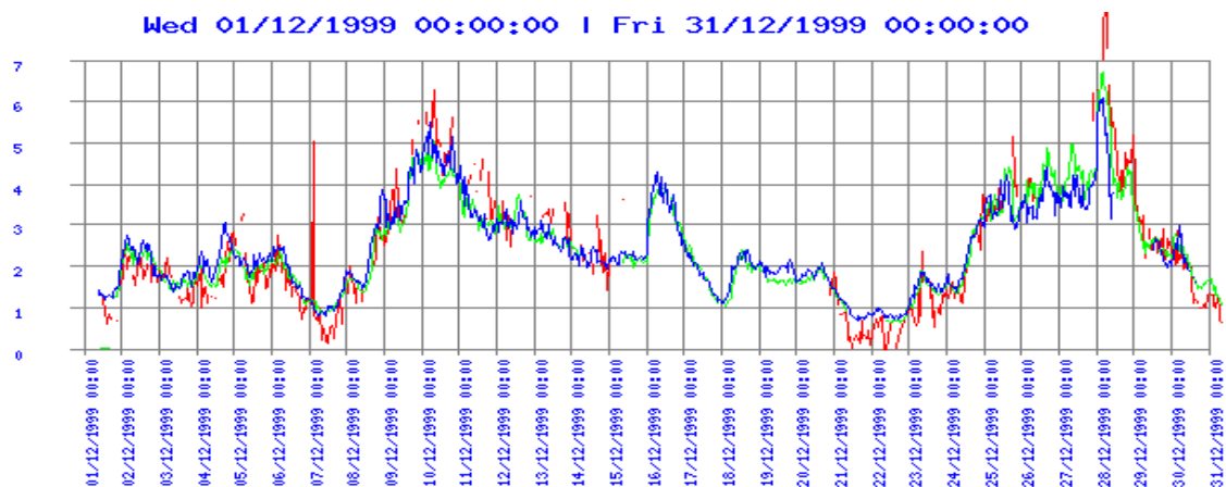
Comparison of significant Wave height propagated from offshore buoy with a coastal buoy
