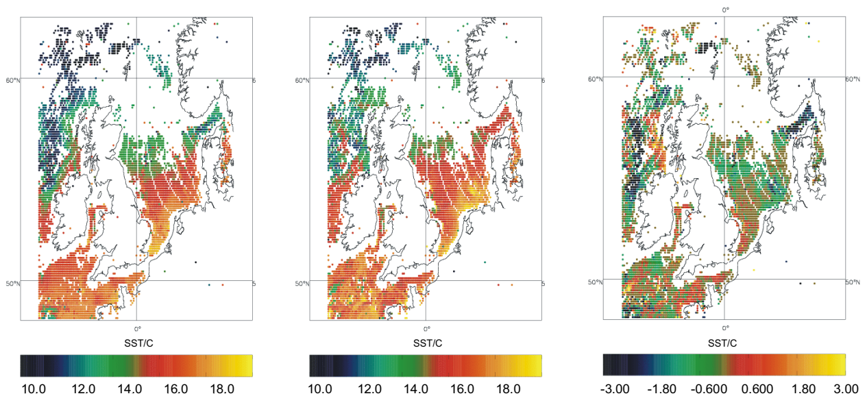
Figure 1: Example of use of monthly composite AVHRR data for shelf seas model validation averaged over August 2000. Left: observed field. Centre: corresponding model field; the model data are extracted to the times and locations of the observations. Right difference (model - observed)
