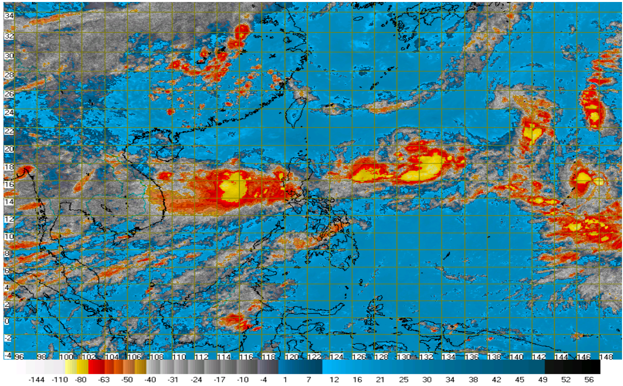
Figure 6: Example Infrared imagery of the Pacific Ocean region
