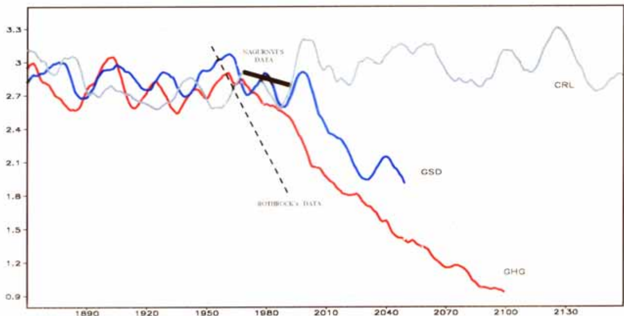
Figure 1: Spatially averaged ice thickness in the Arctic from three simulations with ECHAM-4: control run, forcing by greenhouse gases - GHG, and forcing by greenhouse gases and aerosols - GSD. Data from Nagurny et al (1999) and Rothrock et al (1999) are superimposed.
