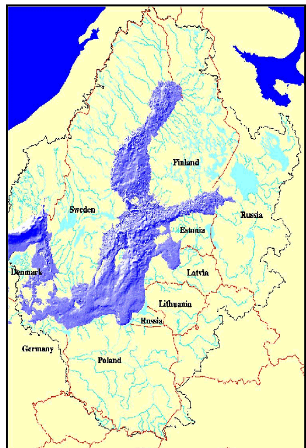
Figure 1: Baltic Sea area (Bottom topography, drainage basins, and political borders)
