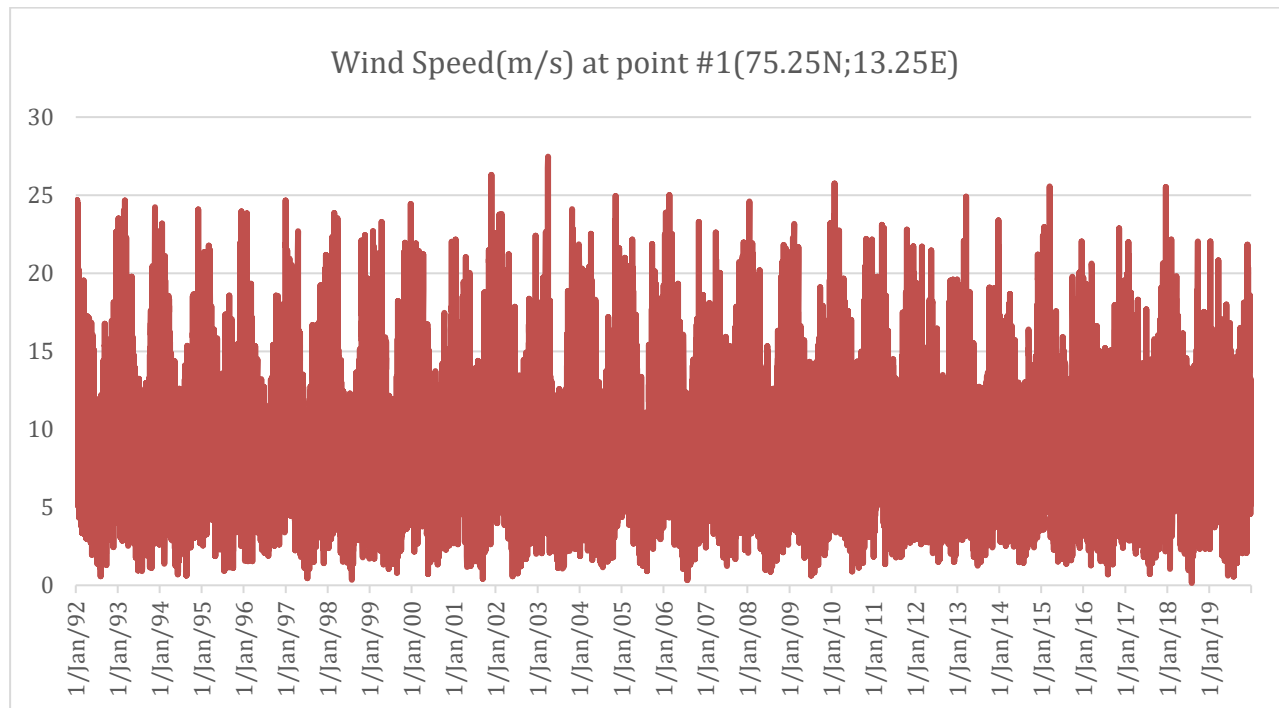
Fig 4.8 Time series of 6-hourly wind speed at point 1 (west of Svalbard).
