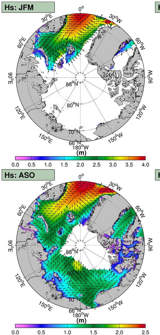
Fig 4.10 January–February–March (JFM) and August–September–October (ASO) seasonal averages of significant wave Height (Hs). From a wave hindcast 1992-2014 (Source: Stopa et al., 2016)
