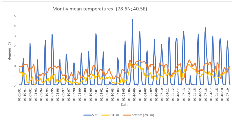
Fig 4.21 Monthly mean temperature at three depths in the Barents Northern point.
