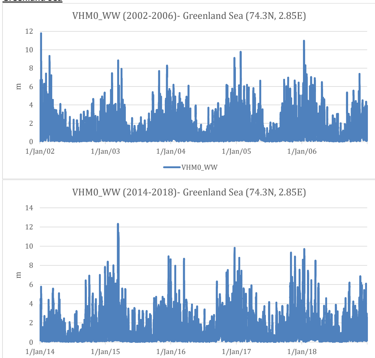
Figure 4.13 Significant wave height (m) for two 5-year periods in the Greenland Sea
