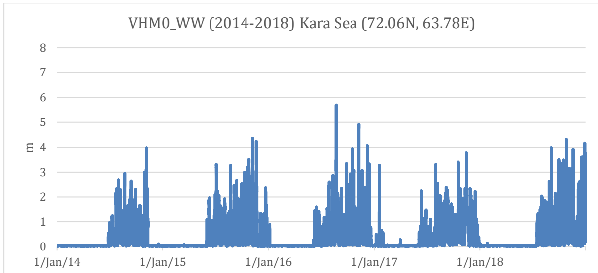
Figure 4.14 Significant wave height (m) for two 5-year periods in the Kara Sea
