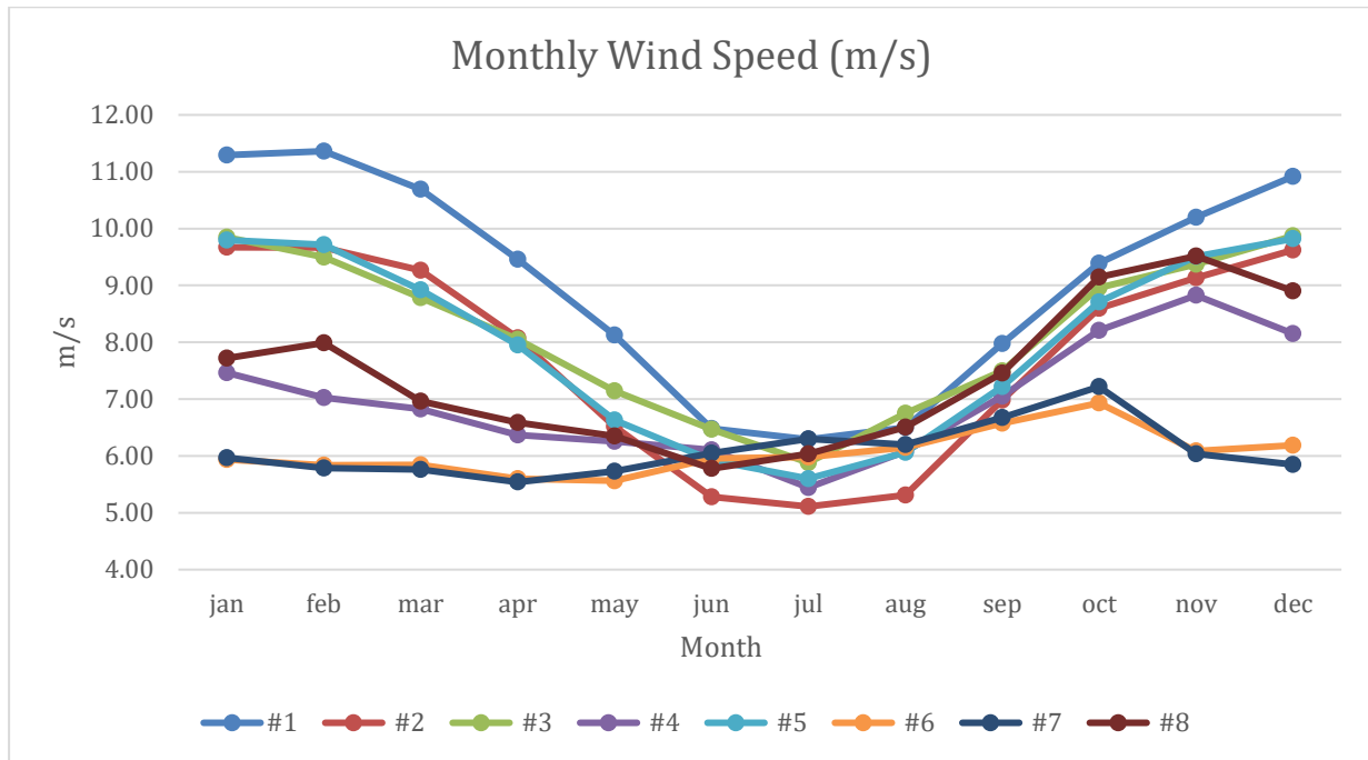
Fig 4.7 Monthly mean wind speeds for the different points in the Arctic. The monthly averages are computed from a 28-years' time series of 6-hourly wind speed dataset.
