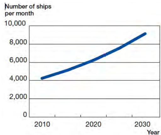
Fig. 22 The increase in number of ships is 2.6% to 5.2% per year until 2030. In the graph the mean value of the increase, 3.9% per year, used when calculating the future growth. (Swedish Environmental Protection Agency, 2008)
