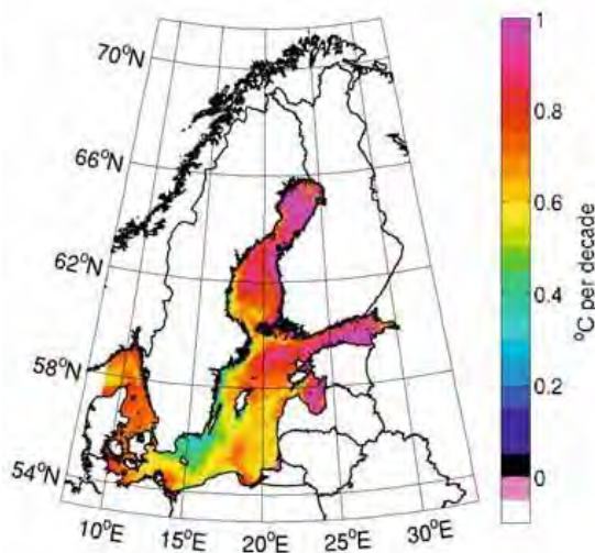
Figure 13. Linear trend of the annual mean sea surface temperature based on infrared satellite data (1990 to 2008) provided by the Federal Maritime and Hydrographic Agency (BSH), Hamburg (Lehmann et al., 2011).
