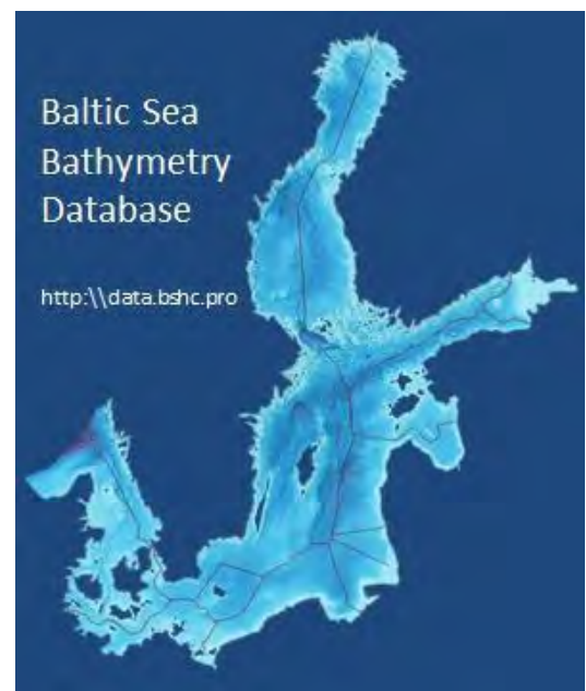
Figure 4 Bathymetry database
