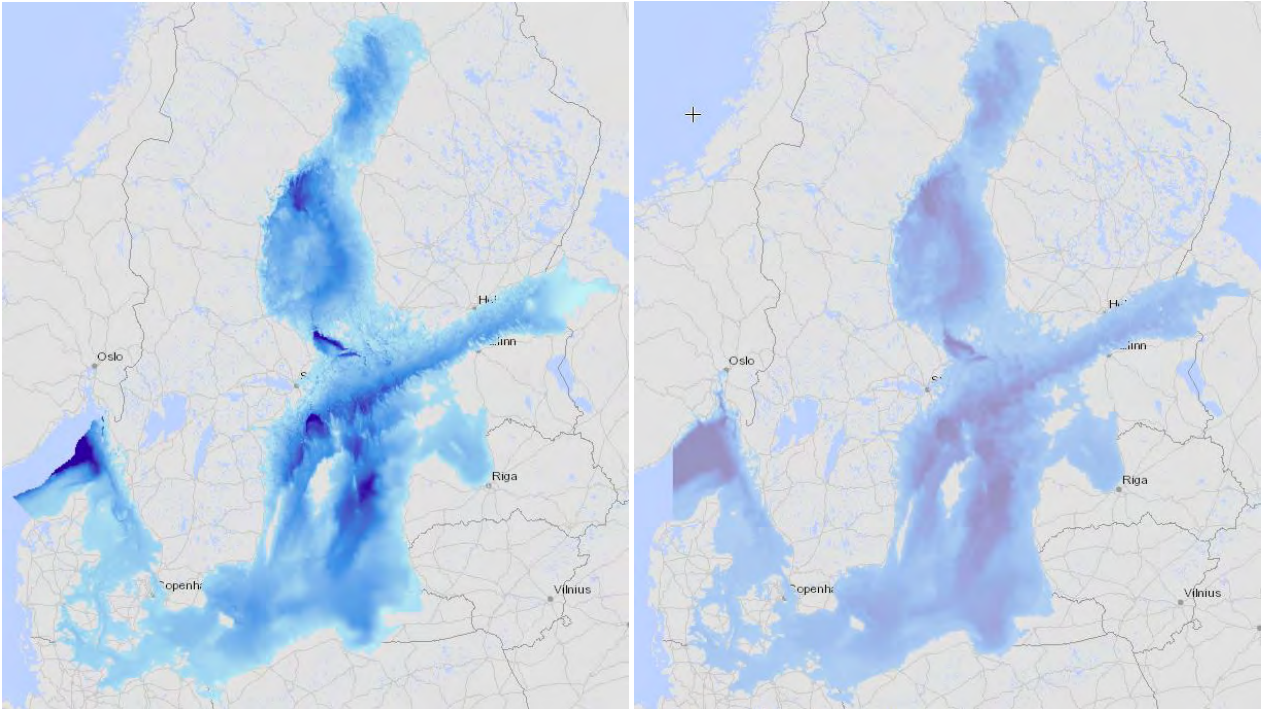
Figure 4.4. Bathymetric based on Bathymetry Data Model (left) and Digital Topography of the Baltic Sea database (Source: Baltic Sea data and map service, 2016)
