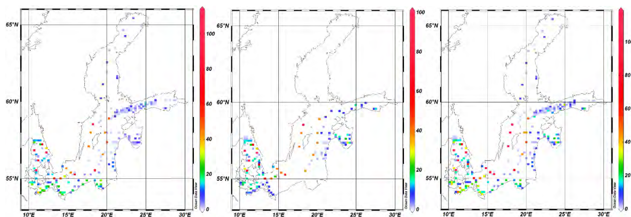
Figure 10.2.3.1. Chlorophyll-a assessment data distribution (sample count per station) for 2005-2014. From left to right: 1) ICES/HELCOM data; 2) EMODnet Chemistry data; 3) ICES/HELCOM and EMODnet Chemistry data pooled. Please note the different scales.
