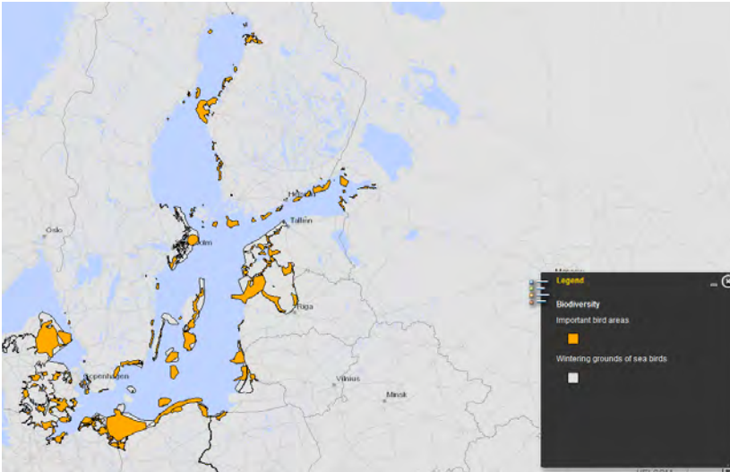
Figure 3.1. Bird areas and wintering bird areas in the Baltic Sea (HELCOM DMS)
