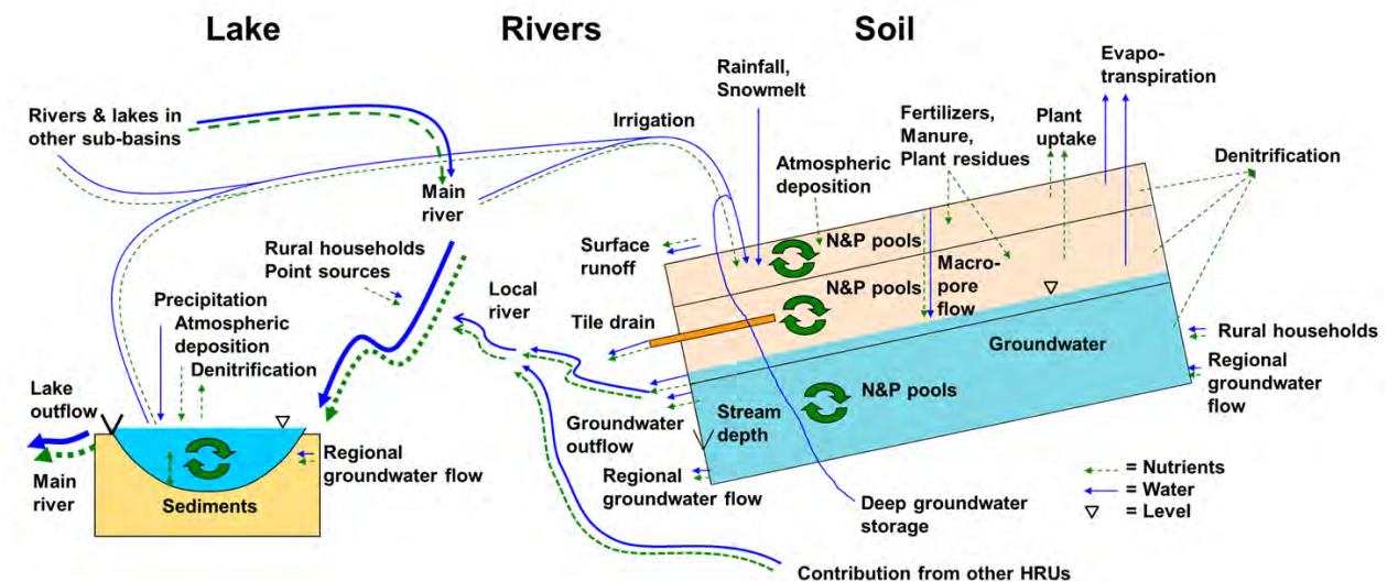
Figure 11.5. Schematic description of HYPE model ( http://www.smhi.se/en/research/research-departments/hydrology/hype-1.7994 )
