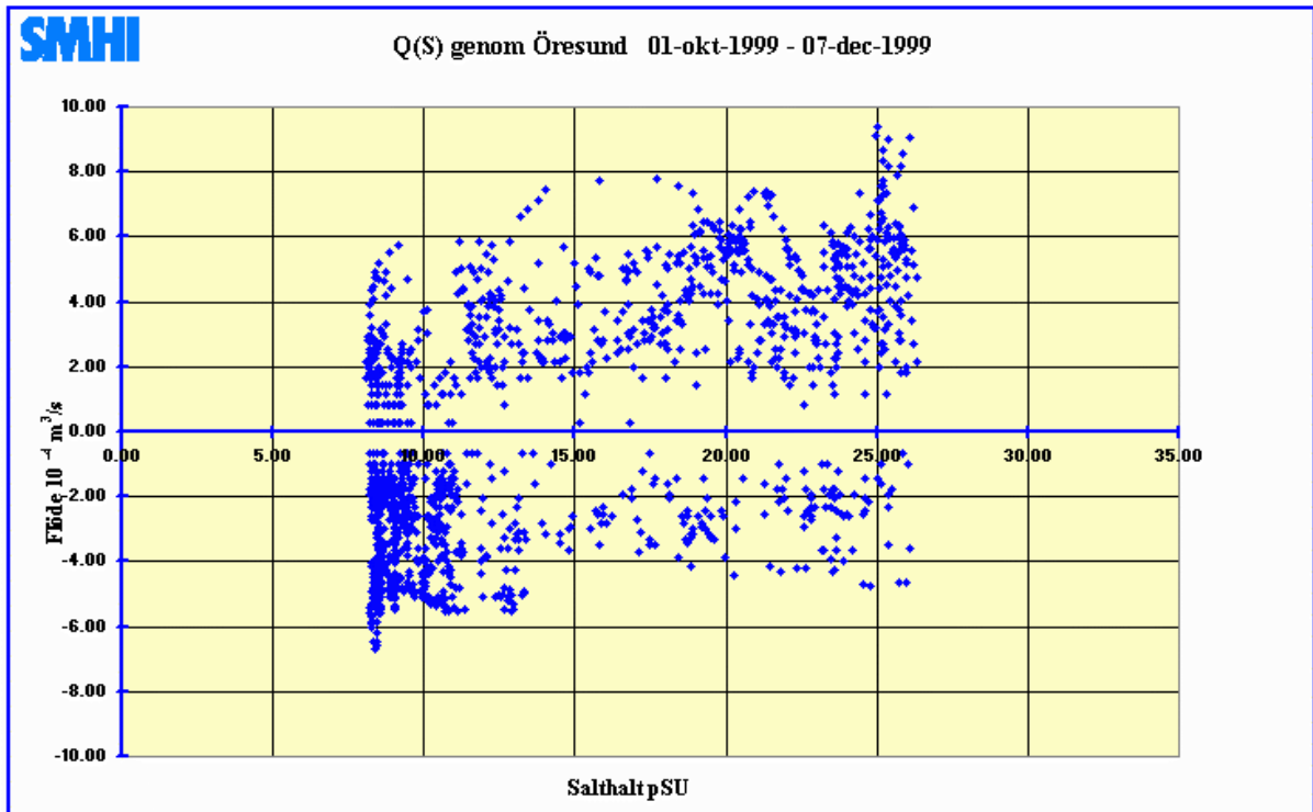
Figure 6. Volume transport ( 10^4 \text{ m}^3/\text{s} ) versus salinity of water flowing in and out of the Baltic Sea during the period 1 October - 7 December 1999. Positive values of Q_s means inflow while negative values means outflow. Real-time updates are available on the SMHI homepage
