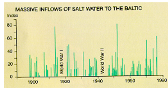
Figure 3. The size of the inflows is characterised by an index based on the duration and mean salinity. High values represent large inflows (from National Atlas of Sweden)
