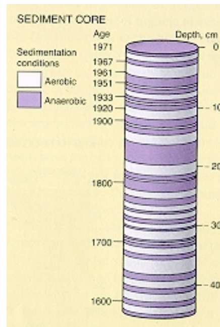
Figure 10c. Samples show that oxygen deficiencies occur regularly in the Baltic Sea (from National Atlas of Sweden).
