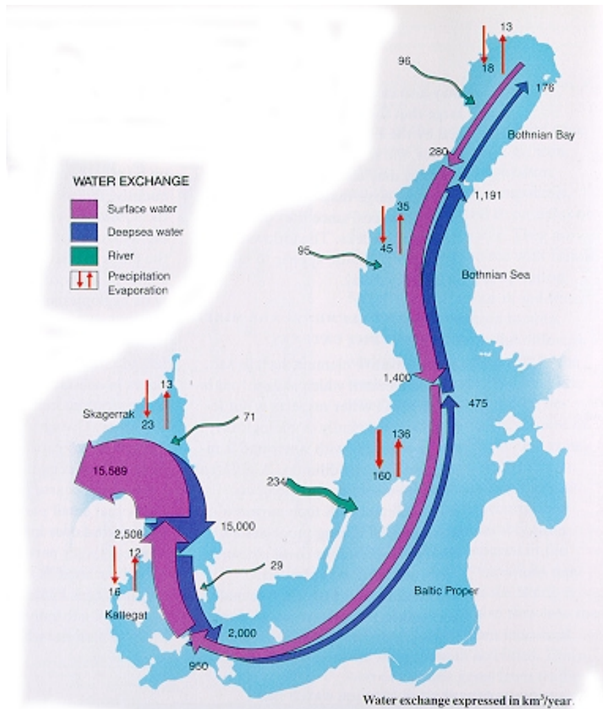
Figure 2. Water exchanges in the Baltic in \text{km}^3/\text{year} . Note that the river inputs are only shown for the Swedish coast. The Evaporation/Precipitation arrows refer to the sea areas within the Swedish sector of the Baltic. The exchanges through the Straits, and the Baltic water flows inwards and outwards, are shown for the whole Baltic (from National Atlas of Sweden).
